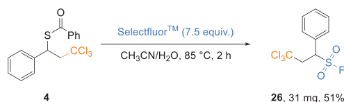
SCHEME 2 | Synthetic application.
